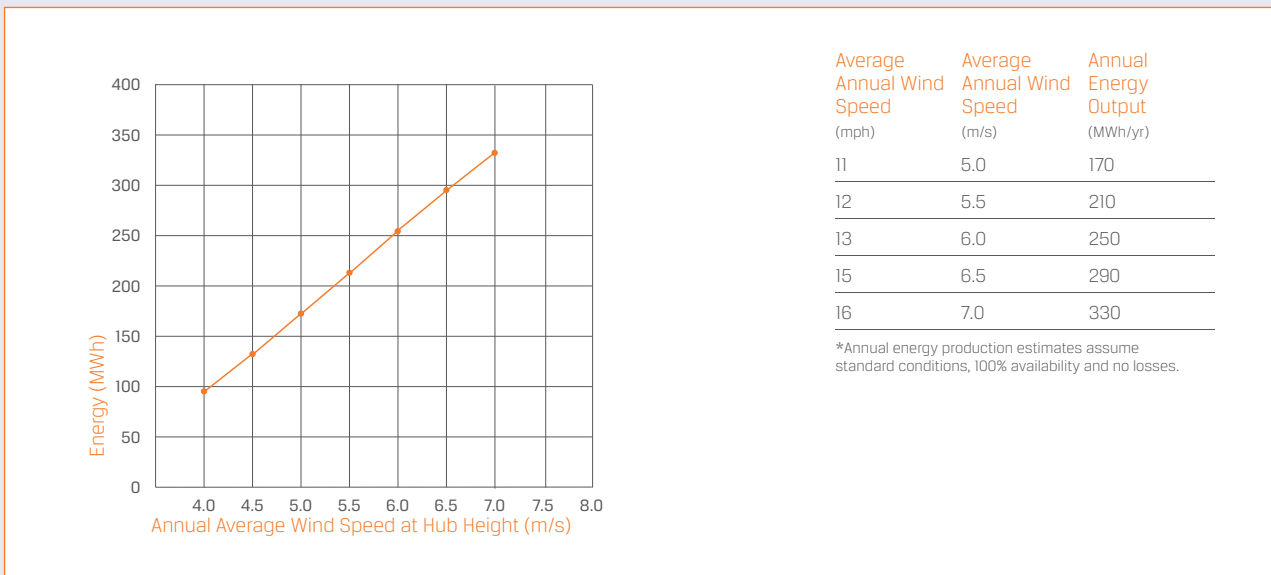
Annual Energy Production*: 24-Meter Rotor Standard Air Density, Rayleigh Wind Speed Distribution
