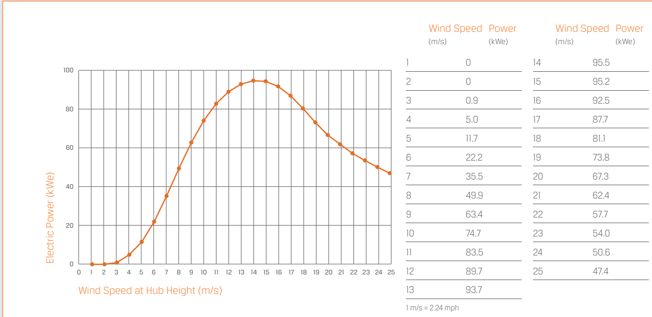
Power Curve: 24-Meter Rotor Standard Air Density (1.225 kg/m 3 )
